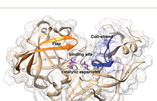
Fig. 2 Flap (resid 67–88) and coil-strand (resid 282–302) regions are two of the common structural features of PAPs. The flap acts as a lid over the catalytic aspartates. Opening of the flap exposes the binding site which enables ligand binding. Figure was created using PDB:1LF4. 13
