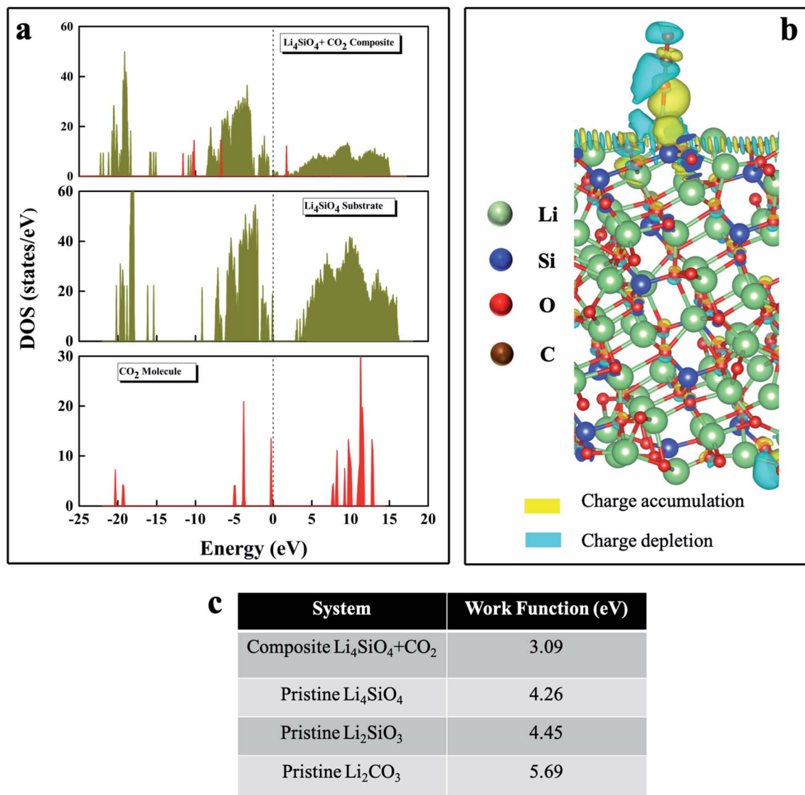
Fig. 8 (a) Density of states plot for CO 2 adsorbed on top of Li 4 SiO 4 . The top panel illustrates the total DOS of the composite systems after adsorption, while the middle and bottom panels represent the DOS of the isolated Li 4 SiO 4 sorbent and CO 2 molecule before adsorption. (b) Charge density distribution between a Li 4 SiO 4 nanosheet and CO 2 molecule. The accumulation and depletion of charge are denoted by yellow and blue color, respectively. The iso-surface value was set to 0.0003 e - Å -3 . (c) Work function and DFT total energies in the bulk form of reactants and products.
