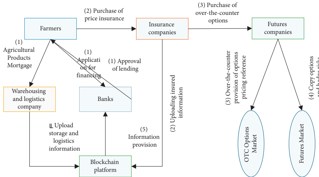
FIGURE 3: Design of blockchain-based ASCF model.
