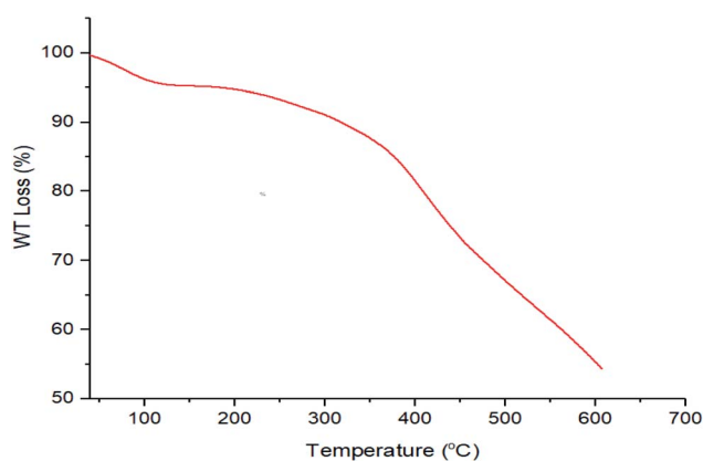
Fig. 8 Thermal gravimetric (TG) analysis of CQDs–N(CH 2 PO 3 H 2 ) 2 .
