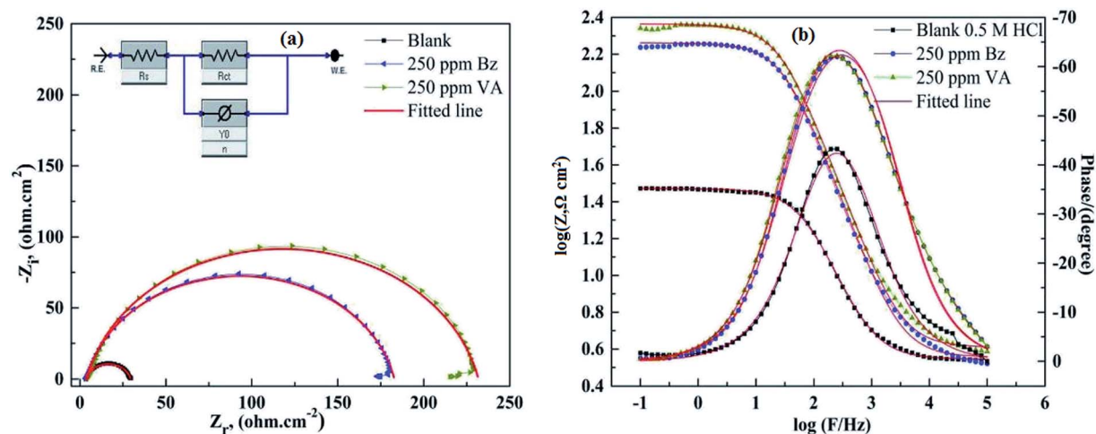
Fig. 4 (a and b) Fitted Nyquist and Bode EIS plots; (dotted) and their fittings (solid lines) for MS in 0.5 M HCl in the absence and presence of optimum concentration of ( Bz ) and ( VA ) at 298 K. The electrochemical equivalent circuit used to fit the impedance spectra (inset).
