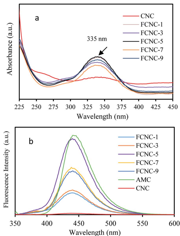
Fig. 5 (a) UV-vis absorption spectra of FCNC aqueous dispersions; (b) fluorescence emission spectra of FCNC aqueous dispersions (excitation wavelength = 335 nm).
