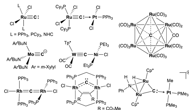
Fig. 1 Examples of metal carbido complexes: neutral terminal carbide, anionic terminal carbide, dative bonding \mu -carbido, metalcarbyne, dimetallacumulene, dimetallo-carbene, trinuclear \mu_3 -carbido, and interstitial carbide.
