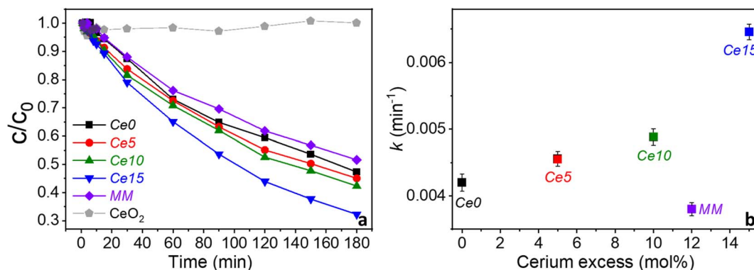
Fig. 6 (a) Thermocatalytic abatement of bisphenol A (initial concentration 10 \text{ mg L}^{-1} ) at 50^\circ \text{C} for perovskites ( 1 \text{ g L}^{-1} ) with excess ceria and the mechanical mixture (MM) and (b) change in kinetic constant ( k ) with increasing excess ceria and comparison with the mechanical mixture. Errors in (a) are smaller than the size of the symbols, whereas in (b) the errors are indicated in the graph for each k value.
