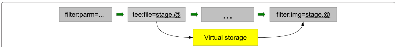
Figure 3 Construction of non-linear pipelines by using the tee filter and virtual storage. Note, the virtual storage is located in main memory.
