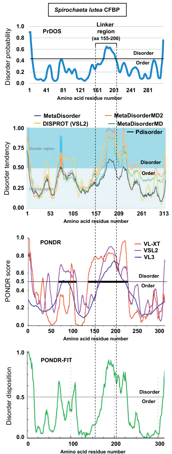
Fig. 3. Comparison of multiple disorder prediction programs and validation of PrDOS. The Spirochaeta lutea CFBP (with a 52-amino acid linker, close to the average linker size in all CFBPs, see Fig. 1), was arbitrarily chosen for disorder prediction by multiple programs that are freely available, as described in Materials and Methods [17, 18]. The PrDOS result (used in the rest of the paper) is compared with the major programs as shown. The default order/disorder cut-off for each program is indicated, and 8% FPR (false positive rate) was chosen for PrDOS, which was translated into 0.43 cut-off, as explained in Materials and Methods. The default terminology and scale of the respective programs were also used to describe their Y-axes. The dotted lines running through all plots bracket the linker sequence (amino acid 155–206) and show the agreement among the programs. Note that in this particular CFBP, the disorder happens to be slanted towards the C-terminal half of the linker. The high spike of disorder in the two termini of the CFBP is a general feature of most proteins, and is to be ignored for this study.
