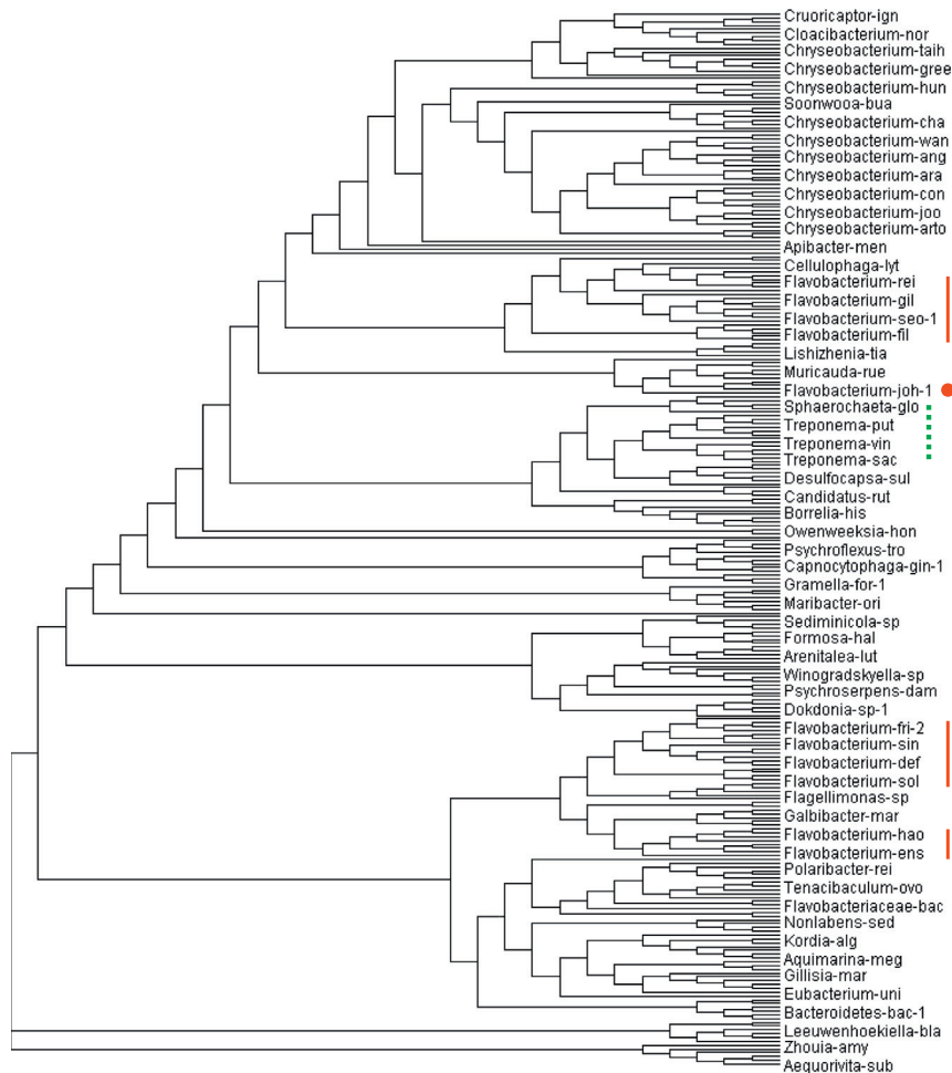
Fig. 2. Phylogenetic relationship among the CFBP linkers. The cladogram tree was generated with 277 linker sequences as described in Materials and Methods. For space constraints, only the major nodes and clade-representative names are shown but this should not detract from the conclusions described in the Results. The scattered Flavobacteria branches are indicated by solid lines and a dot (red in color), the Chryso bacterium clade by double-line (blue in color), and Treponema/Sphaerochaeta ( Spirochaeta ) clades by dotted line (green in color). Note that another spirochete clade, belonging to Borrelia , is also close by (unmarked).
