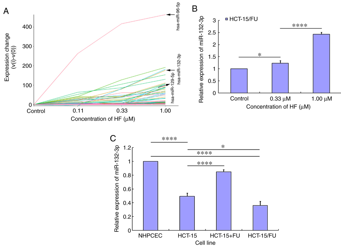
Figure 4. Screening of the miRNA expression profiles in HCT-15/FU cells treated with HF. (A) Using miRNA sequencing analysis and subsequent miRNA trend analysis screening, the expression profiles of human miRNAs in HCT-15/FU cells treated with HF were determined. The expression levels of certain miRNAs were increased in a dose-dependent manner. (B) miR-132-3p expression was increased in HCT-15/FU cells treated with HF in a dose-dependent manner. (C) miR-132-3p expression was downregulated in colorectal cancer HCT-15 and HCT-15/FU cells compared with in NHPCECs. Treatment of HCT15 cells with 5-FU increased the expression levels of miR-132-3p (HCT-15 versus HCT-15/FU) and miR-132-3p expression was lower in HCT-15/FU cells compared with in the corresponding sensitive HCT-15 cells. Experiments were performed in triplicate. * P < 0.05 and **** P < 0.0001 . HF, halofuginone; miR/miRNA, microRNA; NHPCEC, normal human primary colonic epithelial cells; FU, 5-fluorouracil.
