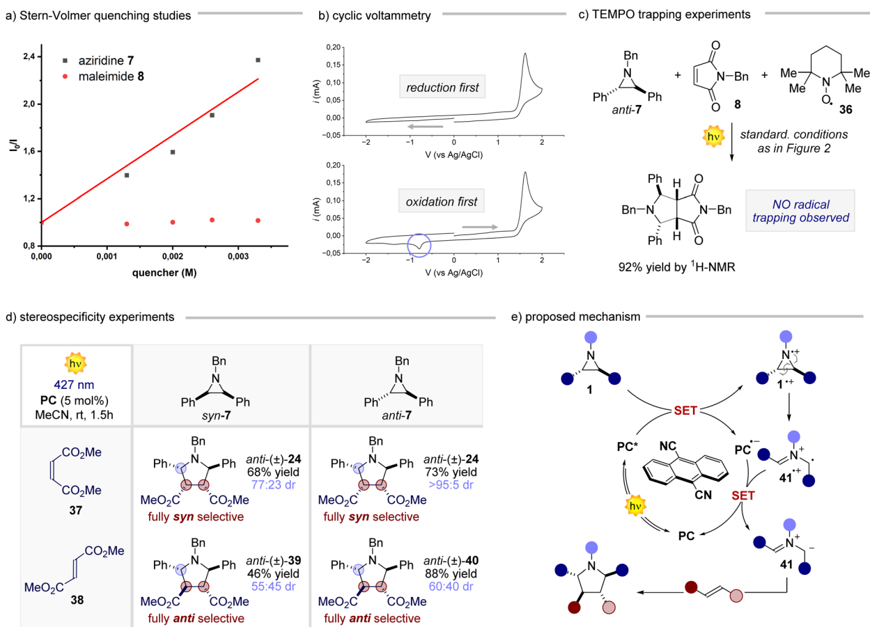
Fig. 3 Mechanistic studies for the photocatalytic reaction of aziridines. (a) Stern–Volmer quenching studies for aziridine 7 and maleimide 8 . (b) Electrochemical analyses of aziridine 7 . (c) TEMPO trapping experiments for the model reaction involving compounds 7 and 8 . (d) Stereospecificity experiments between syn - 7 , anti - 7 maleate 37 and fumarate 38 . (e) Proposed mechanism for the photocatalytic reaction of aziridines with olefins.
