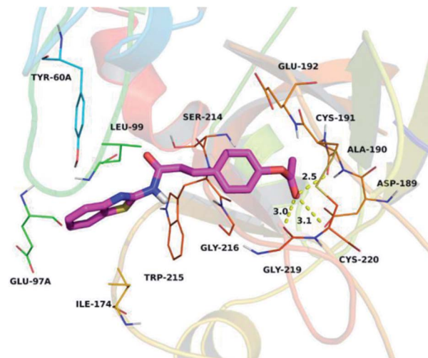
Fig. 5 Compound Q2 docking into the thrombin binding pocket.
