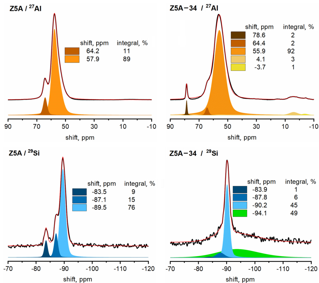
Figure 4. 27 Al and 29 Si MAS NMR spectra of Z5A and Z5A-34 (black lines = measured spectra, red lines = modeled spectra, color filled areas under the curve = individual contributions to the modeled spectra).
