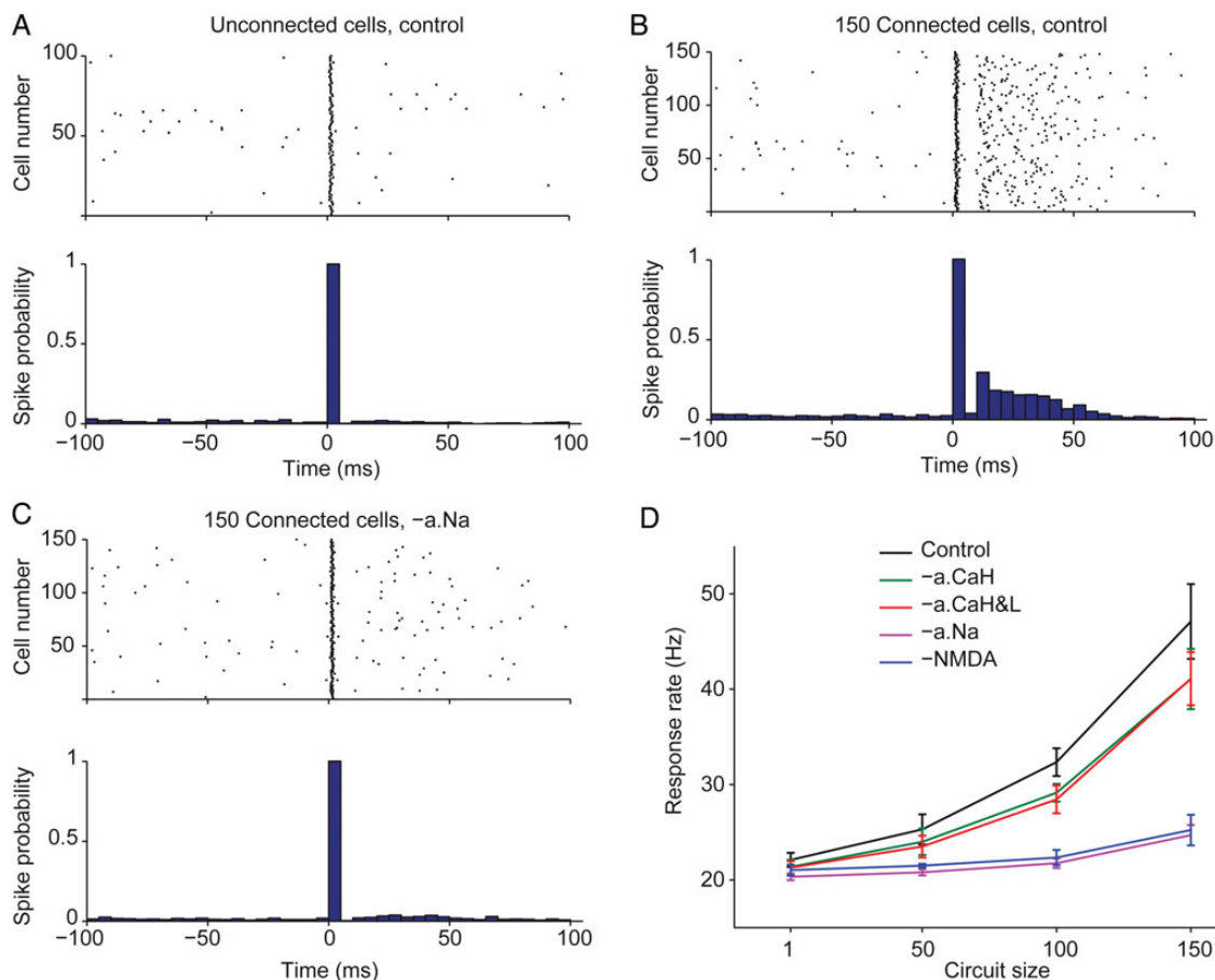
Figure 2. Modulation of response rate by recurrent activity and dendritic excitability. (A) An example raster plot (top) and PSTH (bottom) of the firing of single (unconnected) cells in response to brief suprathreshold somatic/thalamic input at t=0 (stimulus as in Fig. 1B). (B) Example raster plot (top) and PSTH (bottom) for the response to somatic input in microcircuits of N=150 cells, all receiving brief suprathreshold somatic input at t=0 . (C) Same as in (B), except that apical dendritic \text{Na}^+ channels in modeled cells were removed (denoted: -a.Na). (D) Response rate of cells in microcircuits of size N=1-150 cells, in control condition as in (B) (black curve) and when removing particular apical dendritic channels (high-voltage-gated \text{Ca}^{2+} channels, green curve; both high- and low-voltage-gated \text{Ca}^{2+} channels, red curve; \text{Na}^+ channels, purple curve) or NMDA receptors on both basal and apical dendrites (blue curve). The instantaneous rate was measured in a time window of 50 ms following stimulus onset.
