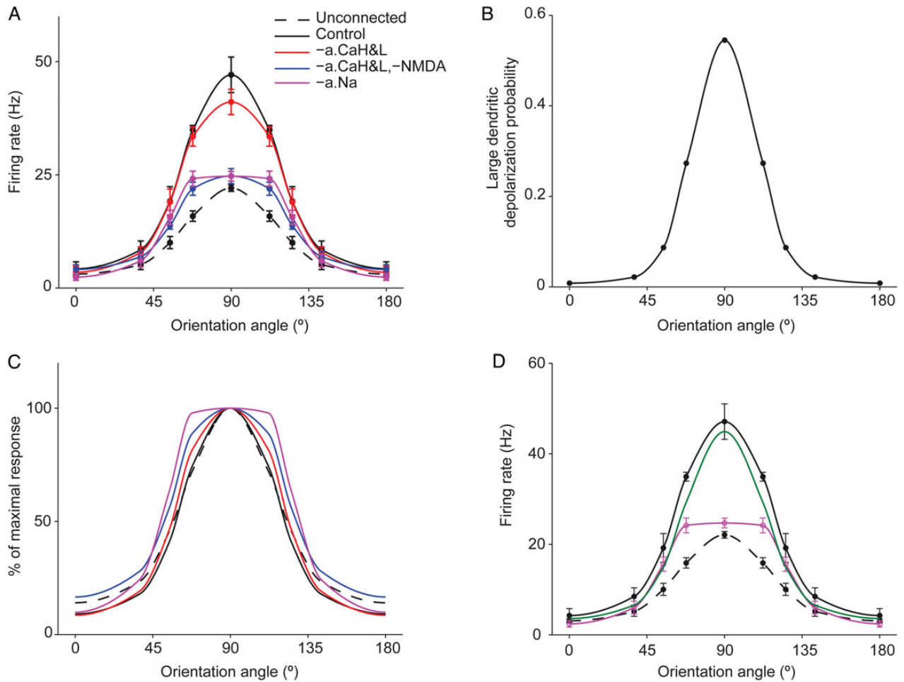
Figure 6. Dendritic excitability and recurrent activity amplify response to thalamic input while maintaining selectivity. (A) The average response in microcircuits of 150 cells (solid curves) or in unconnected cells (dashed black curve) to different somatic pulse amplitudes, reflecting different stimulus orientations (see Materials and Methods). Control conditions are depicted by the black curves whereas color curves are for the cases when dendritic \text{Ca}^{2+} or \text{Na}^{+} channels, or also NMDA receptors were removed. (B) Normalized response curves taken from (A). (C) The probability of large dendritic depolarizations in microcircuits of 150 cells increased with stimulus orientation towards the preferred orientation ( 90^\circ ). Large dendritic depolarization was defined to be the case when the dendritic voltage integral at the main apical bifurcation was >800 mV ms. (D) The predicted response rate in microcircuits of 150 cells based on the probability of obtaining large dendritic depolarization, as a function of orientation (given in C) is shown by the green line. Purple and black curves are as in (A).
