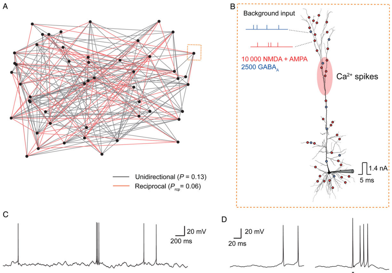
Figure 1. Simulated TTCs microcircuits. (A) An exemplar microcircuit of 50 cells. Connection probabilities between cells were 0.13 for unidirectional connections (black edges), and 0.06 for reciprocal connections (red edges). Reciprocal excitatory synaptic connections were 1.5 times stronger than unidirectional connections. (B) An example of a modeled TTC, with its detailed morphology, receiving a background Poisson input with 10 000 excitatory synapses (red) and 2500 inhibitory (blue) synapses (see Materials and Methods). On top of this background input, all cells in the microcircuit were simultaneously stimulated by a brief somatic current input of 1.4 nA and 5 ms duration (black electrode), mimicking a brief perisomatic thalamic input. In addition to firing somatic Na + APs, the TTC model was capable of generating dendritic Ca 2+ spikes at the apical “hot zone” (shaded red ellipse). (C) Spontaneous firing of an exemplar single (isolated) TTC in response to the background synaptic input. (D) Voltage traces of another example cell, from a microcircuit of 150 cells, firing spontaneously (2 spikes, left) and in response to simultaneous somatic input to all network cells (4 spikes, right). Stimulus is indicated by black bar below the voltage trace.
