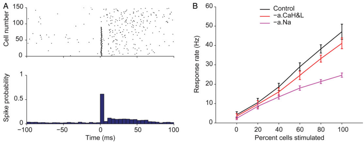
Figure 5. Microcircuit response to a partial thalamic input. (A) Example raster plot (top) and PSTH (bottom) for the response to somatic/thalamic input given to 60% of the cells in microcircuits consisting of 150 cells. (B) The response rate in microcircuits of 150 cells as a function of the percent of cells stimulated, in control conditions (black curve) and when dendritic \text{Ca}^{2+} or \text{Na}^{+} channels were removed (red and purple curves).
