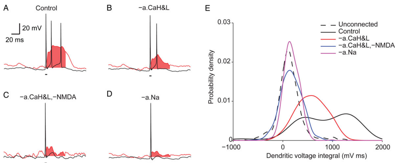
Figure 3. Microcircuit response involves strong dendritic nonlinearities. (A) Voltage traces at the soma (black) and at the apical main bifurcation (650 \mu\text{m} from the soma, red, see scheme in Fig. 1B) of an exemplar cell. The cell was part of a microcircuit of size N = 150 cells, receiving a brief suprathreshold somatic input to all circuit cells in control conditions. Somatic stimulus at t = 0 is indicated by black bar below the trace. The area under the dendritic voltage response, for t = 0 –50 ms, is shaded in red. (B–D) Same as (A), but for the cases when the dendritic \text{Ca}^{2+} channels were removed (B), or also NMDA receptors were removed (C), or only dendritic \text{Na}^+ channels were removed (D). (E) Distribution of the integral of the membrane depolarization at the apical main bifurcation over the 50 ms time window in all cells from microcircuits of 150 cells from 4 different randomized simulations ( n = 600 cells for each curve, see Materials and Methods), receiving simultaneous somatic input, under control conditions (solid black curve), when dendritic \text{Ca}^{2+} channels were removed (red curve), when also NMDA channels were removed (blue curve), or when only dendritic \text{Na}^+ channels were removed (purple curve). The distribution for unconnected cells under control conditions is shown by the dashed black curve ( n = 400 cells). The bimodal distribution for the solid black curve indicates nonlinear dendritic events.
