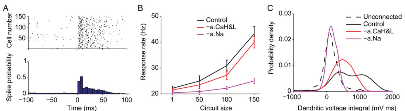
Figure 4. Modulation of network response by recurrent activity and dendritic excitability is robust to temporal noise in the thalamic input. (A) Raster plot (top) and PSTH (bottom) for microcircuits of 150 cells, receiving brief suprathreshold somatic input, with a random jitter of 0–10 ms in the onset of the somatic stimulus. (B) Response of cells in microcircuits of size N=1 –150 receiving somatic input with 0–10 ms jitter, in control conditions (black curve) and when dendritic Ca 2+ or Na + channels were removed (red and purple curves). (C) Distribution of voltage integral at the main apical bifurcation in all cells from microcircuits of 150 cells ( n=600 ), receiving jittered somatic input, under control conditions (solid black curve) and when dendritic Ca 2+ or Na + channels were removed (red and purple curves). The distribution of dendritic integral for unconnected cells is given by the dashed black curve ( n=400 ).
