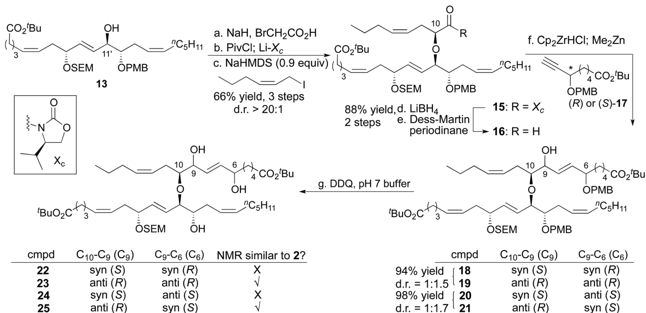
Scheme 3 Synthesis of fatty acid portion of nigriganoside. (a) NaH, BrCH 2 CO 2 H, THF/DMF = 2/1, 0 °C–rt, 91%. (b) PivCl, Et 3 N, Et 2 O, 0 °C; Li-X c , THF, rt, 91%. (c) (Z)-1-iodohex-2-ene, NaHMDS (0.9 equiv.), THF, –78 °C, 79%, d.r. > 20 : 1, +9% recovered starting material. (d) LiBH 4 , MeOH, THF, 0 °C, 94%. (e) Dess–Martin periodinane, NaHCO 3 , CH 2 Cl 2 , 0 °C, 94%. (f) (+)-17 or (–)-17, Cp 2 ZrHCl; Me 2 Zn; 16, CH 2 Cl 2 /toluene, –78–0 °C. (g) DDQ, pH7 buffer/CH 2 Cl 2 , 0 °C–rt.
