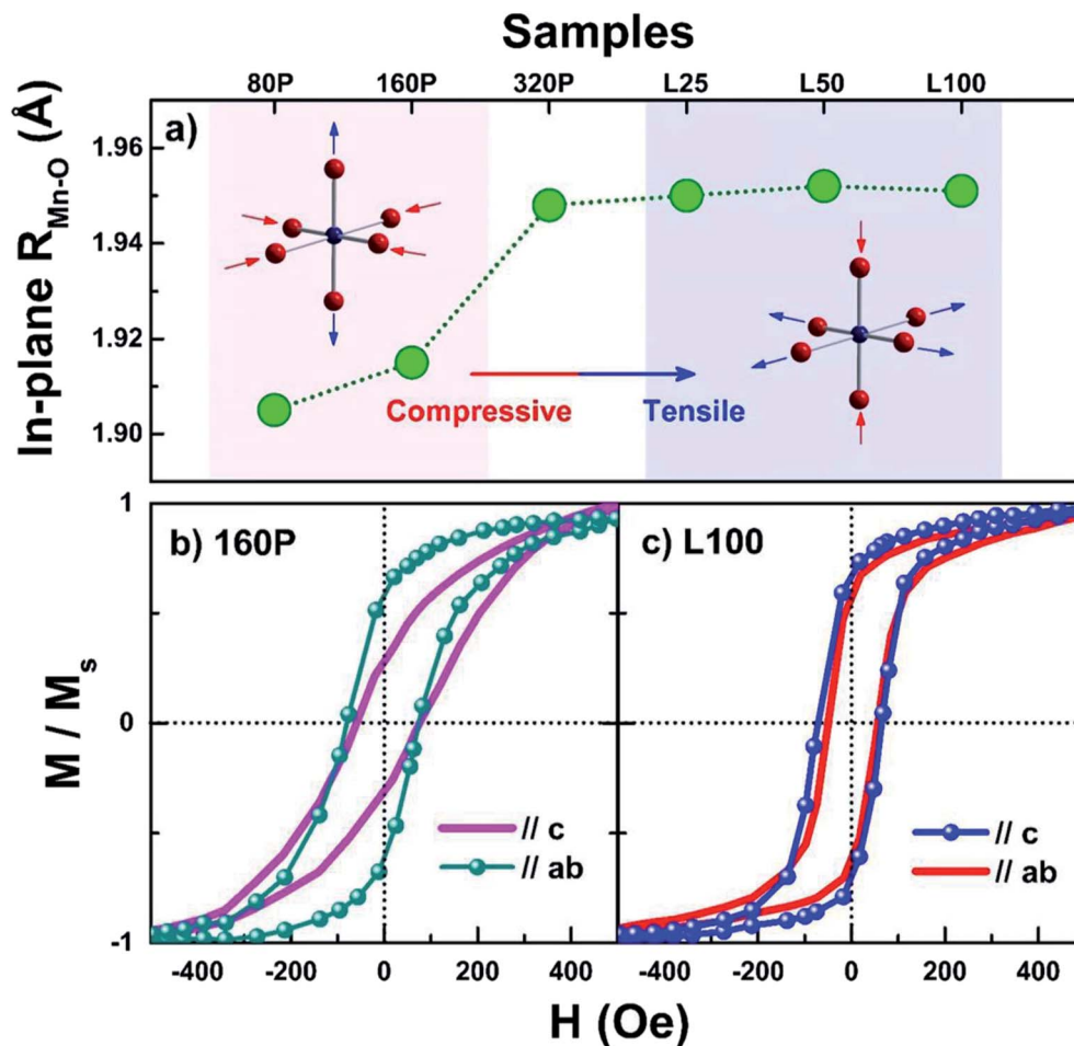
Fig. 4 (a) In-plane Mn–O bond distance as a function of samples. The normalized in-plane and out-of-plane magnetization curves for (b) 160P and (c) L100.
