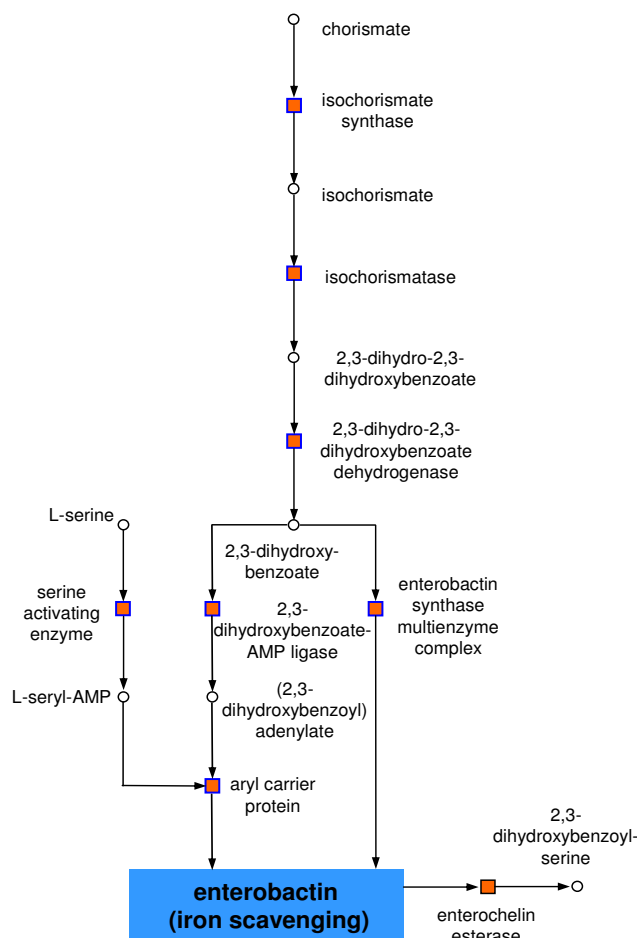
Figure 6 Iron processing in an anaerobic environment. Iron is scavenged by E. coli using enterobactin, whose biosynthesis (blue bordered nodes) was down-regulated. For box colours see Figure 4.
