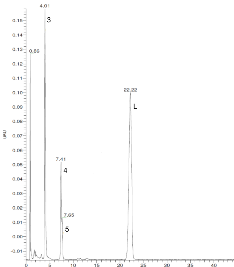
Figure 2 UV chromatogram of a mixed sample illustrating lumefantrine N-oxide, lumefantrine DBK and desbenzyl derivative and lumefantrine. UV chromatogram of a mixed sample illustrating lumefantrine N-oxide (3), DBK (4) and desbenzyl lumefantrine derivative (5) and lumefantrine (L).
