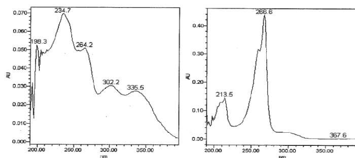
Figure 4 UV spectra recorded for lumefantrine (left) and DBK (right) showing the observed wavelength of maximum absorption. DAD-UV spectra of lumefantrine (left) and DBK (right).
