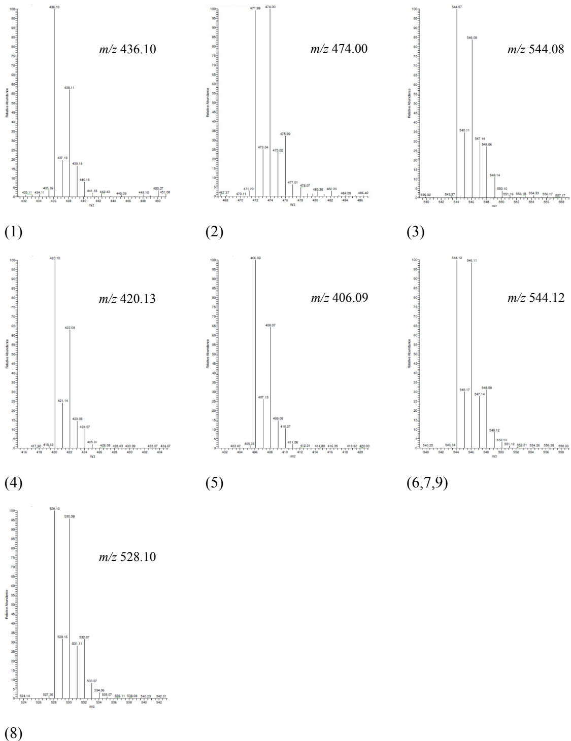
Figure 3 Isotopic-distribution mass spectra of lumefantrine related impurities with the most abundant m/z observed. Isotopic-distribution mass spectra of lumefantrine related impurities: (1) Desbenzyketo N-oxide; (2) Monodesbutyl derivative; (3) Lumefantrine N-oxide; (4) Desbenzyketo derivative; (5) Desbenzyl derivative; (6,7,9) Oxide of lumefantrine and (8) Impurity A (USP/Ph.Int).
