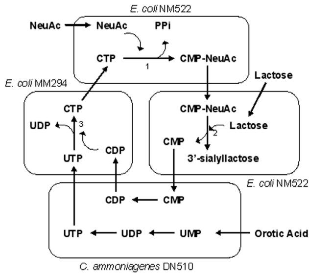
Figure 5 Metabolic pathway for CMP-NeuAc synthesis from NeuAc and orotic acid [14]. Enzymes – 1: CMP-NeuAc synthetase (NeuA), 2: α2,3-sialyltransferase, 3: CTP synthetase (PyrG).
