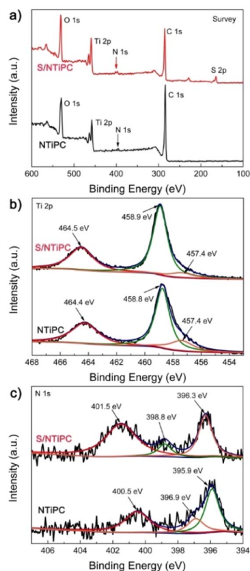
Fig. 3 XPS spectra of NTiPC and S/NTiPC composites: (a) survey scan; (b) Ti 2p; and (c) N 1s.
