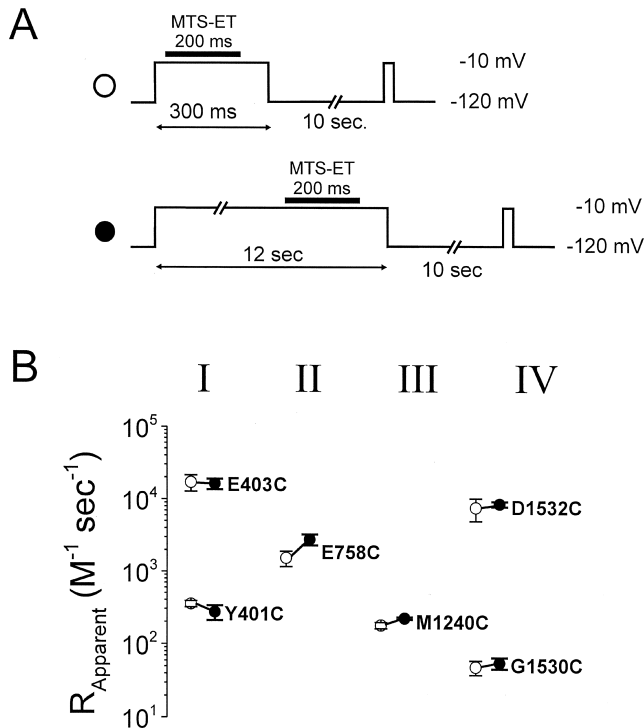
FIGURE 5. No state-dependent change of cysteine modification rate was seen in the six mutants studied. (A) Schematic representation of the pulsed MTS-ET application protocols. Modification rates for fast-inactivated channels were assayed by exposing outside-out patches to MTS-ET for 200 ms, beginning 20 ms into the 300 ms conditioning pulse (top protocol, open circles). To measure the modification rate of slow-inactivated channels, patches were exposed to MTS-ET beginning 10.5 s after the onset of a 12 s conditioning pulse (bottom protocol, filled circles). All conditioning pulses were to -10 mV, and a gap of 10 s at -120 mV to allow for full recovery from inactivation was inserted before a test pulse to -20 mV to measure remaining peak I_{Na} . This cycle was repeated until maximal modification in each patch had taken place. (B) Comparison of modification rates of cysteines in each of the four domains measured under conditions in which channels were predominantly fast- or slow-inactivated. The mean and SEM of these rates are plotted by domain location for each mutant, with rates for the two states of the channel connected by a line. The numerical values are listed in Table II.
