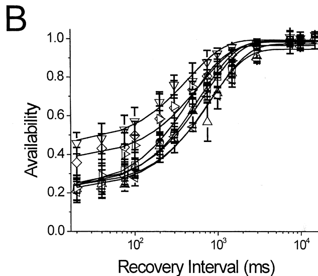
FIGURE 2. Introduction of cysteine missense mutations into informative P-region sites has little or no effect on the recovery kinetics of fast- or slow-inactivation. All measurements were made in excised outside-out macropatches held under perfusion with control bath solution. Conditioning pulses to -10 mV of 40 ms or 3 s duration were used to induce fast and slow inactivation, respectively, (A, inset). (A) Recovery from fast inactivation at -120 mV was unchanged between cysteine substitution mutants and wild-type. (B) Recovery from slow inactivation at -120 mV was not affected by introduction of cysteine residues at most informative sites. For E758C mutant channels, a modest acceleration in the time course of recovery was observed.
