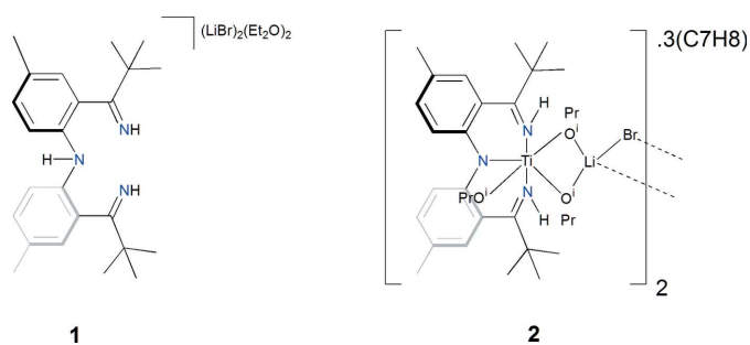
Figure 1 The molecular structure of [NNN] H 3 ( 1 ), with C-bound H atoms and minor components of disorder removed for clarity. Symmetry code: (A) -x + 1, y, -z + \frac{1}{2} .
