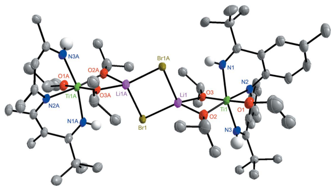
Figure 2 The molecular structure of the dinuclear {[NHNH]Ti(OiPr) 3 (LiBr) 2 ] 2 complex ( 2 ), with all hydrogen atoms bound to C atoms removed for clarity. Symmetry code: (A) -x, -y + 1, -z + 1 .
