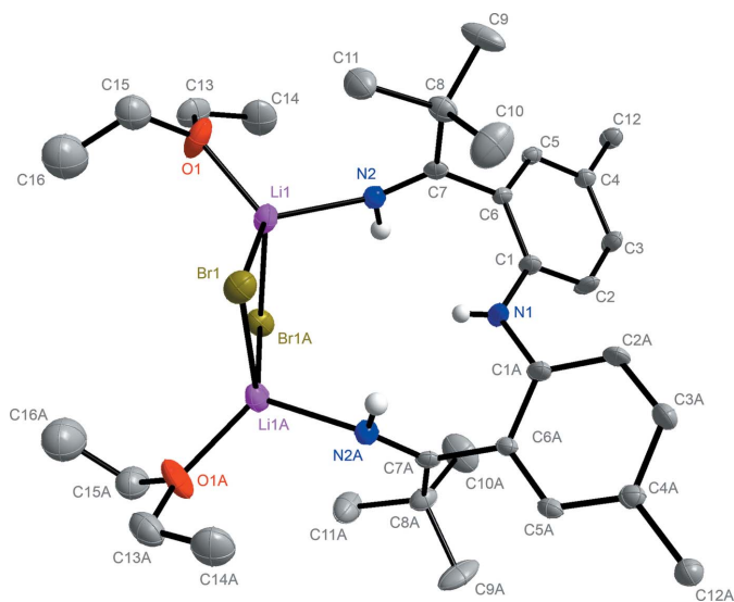
Figure 1 The molecular structure of [NNN] H 3 ( 1 ), with C-bound H atoms and minor components of disorder removed for clarity. Symmetry code: (A) -x + 1, y, -z + \frac{1}{2} .
