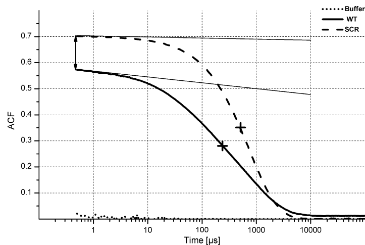
Fig 8. DLS experiment of WT A\beta 1–40 and SCR A\beta 1–40. Representative autocorrelation function (ACF), directly adapted from dynamic light scattering data obtained for WT A\beta 1–40 (line) and SCR A\beta 1–40 (dashes). The autocorrelation function decays in the range of 1 down to 0, and the gap remaining to 1 observed at the shortest correlation time is indicative for the existence of monomeric or low-order oligomers, which remain undetectable. The short-correlation-time asymptote of ACF is marked by thin solid lines. The mid-point of an ACF decay is marked by the cross.
