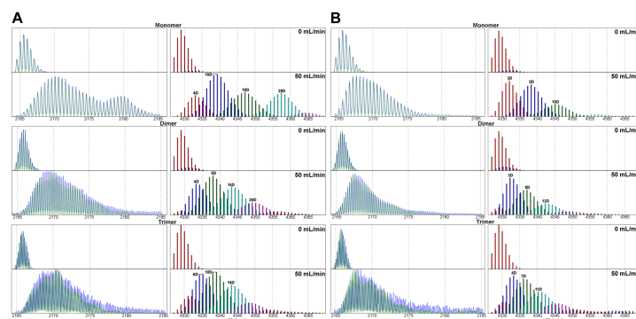
Fig 4. Analysis of the isotopic envelopes after gas-phase HDX-MS for selected signals of species bearing the same charge per monomer, namely MON 2+ , DIM 4+ and TRI 6+ (2164–2185 m/z range) of WT A \beta 1–40 (A) and SCR A \beta 1–40 (B). Left panels— isotopic envelopes corresponding to MON 2+ (upper panels), DIM 4+ (middle panels), TRI 6+ (lower panels), for make-up gas flow 50 mL/min in the presence of ND 3 /D 2 O reagent. Right panels—decomposition of the experimental isotopic envelope into a family of isotopic envelopes of FWHM, expected for a single conformational state. The spectra were recalculated from m/z domain, (shown in left panels) to the domain of molecular mass of a monomeric unit in an oligomer (shown in right panels). Results of replicates of this experiments are shown in Figure C in S1 Appendix.
