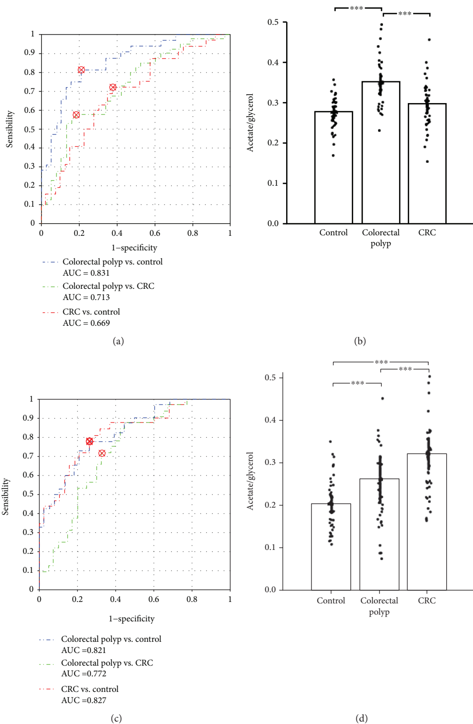
FIGURE 5: Diagnostic potential for colorectal polyp and CRC by rates (acetate/glycerol, lactate/citrate) from serum data. (a) ROC curves of the rate of acetate/glycerol (colorectal polyp vs. control with a 0.831 AUC, colorectal polyp vs. CRC with a 0.713 AUC, and CRC vs. control with a 0.669 AUC); (b) rate of acetate/glycerol in serum samples from control, colorectal polyp, and CRC patients; (c) ROC curves of the rate of lactate/citrate (colorectal polyp vs. control with a 0.821 AUC, colorectal polyp vs. CRC with a 0.772 AUC, and CRC vs. control with a 0.827 AUC); (d) rate of lactate/citrate in serum samples from control, colorectal polyp, and CRC patients. ^{***}p < 0.001 .
