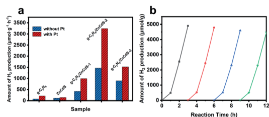
Fig. 5 (a) Photocatalytic hydrogen production rates of g\text{-C}_3\text{N}_4 , ZnCdS, and g\text{-C}_3\text{N}_4/\text{ZnCdS} with (red bars) and without (blue bars) Pt cocatalyst; (b) recycling performance of CN/ZCS-2 (each color represents one test cycle).
