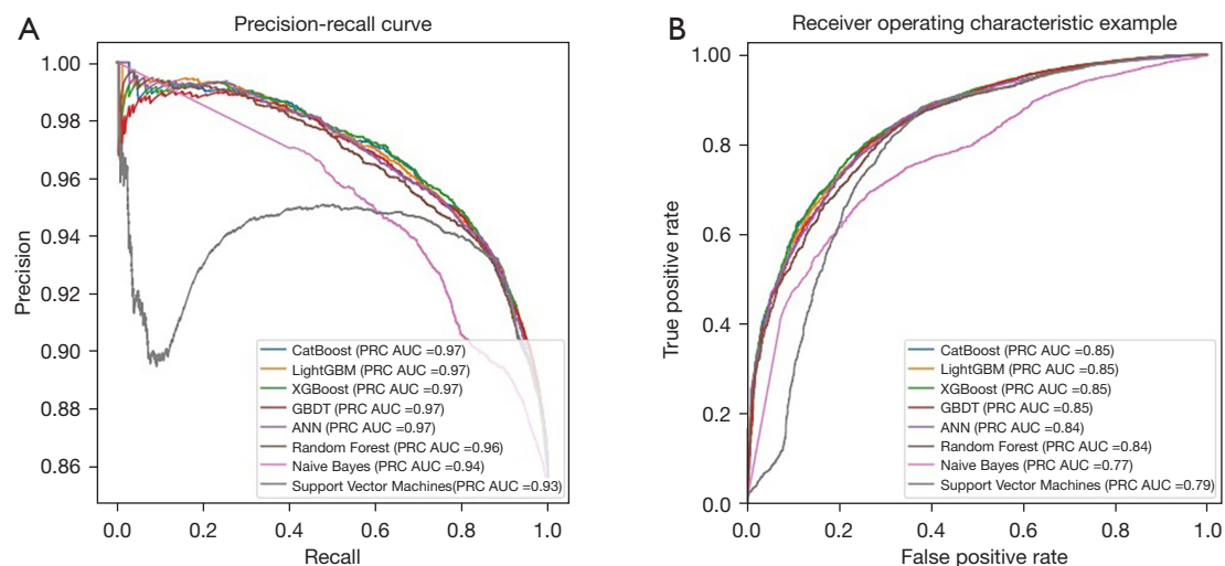
Figure 2 Visual representation of model performance based on 8 algorithms trained by the complete dataset. (A) The precision-recall curve. (B) The ROC curve. When the AUC is closer to 1, the performance of the model classification and prediction is better. ROC, receiver operating characteristic; AUC, area under the ROC curve.
