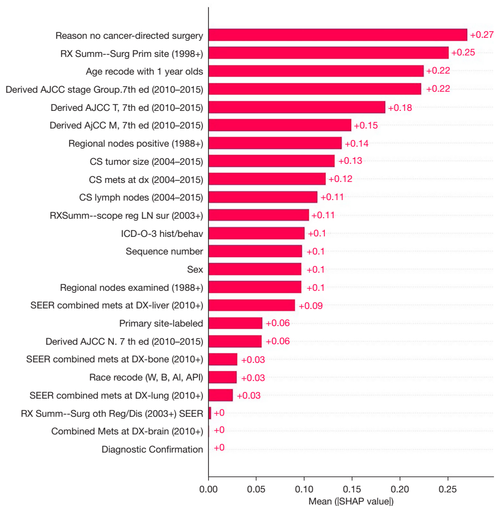
Figure 3 SHAP feature importance measured as the mean absolute SHAP value. SHAP, SHapley Additive exPlanations.
