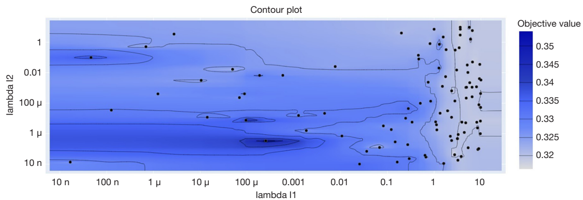
Figure 1 An example of hyperparameter tuning of the LightGBM model. There are 100 dots in the picture. Each dot represents a trial. The shade of blue indicates the range of the objective value. The objective function is defined as the average logistic loss of the 5-fold cross-validation of the LightGBM model.
