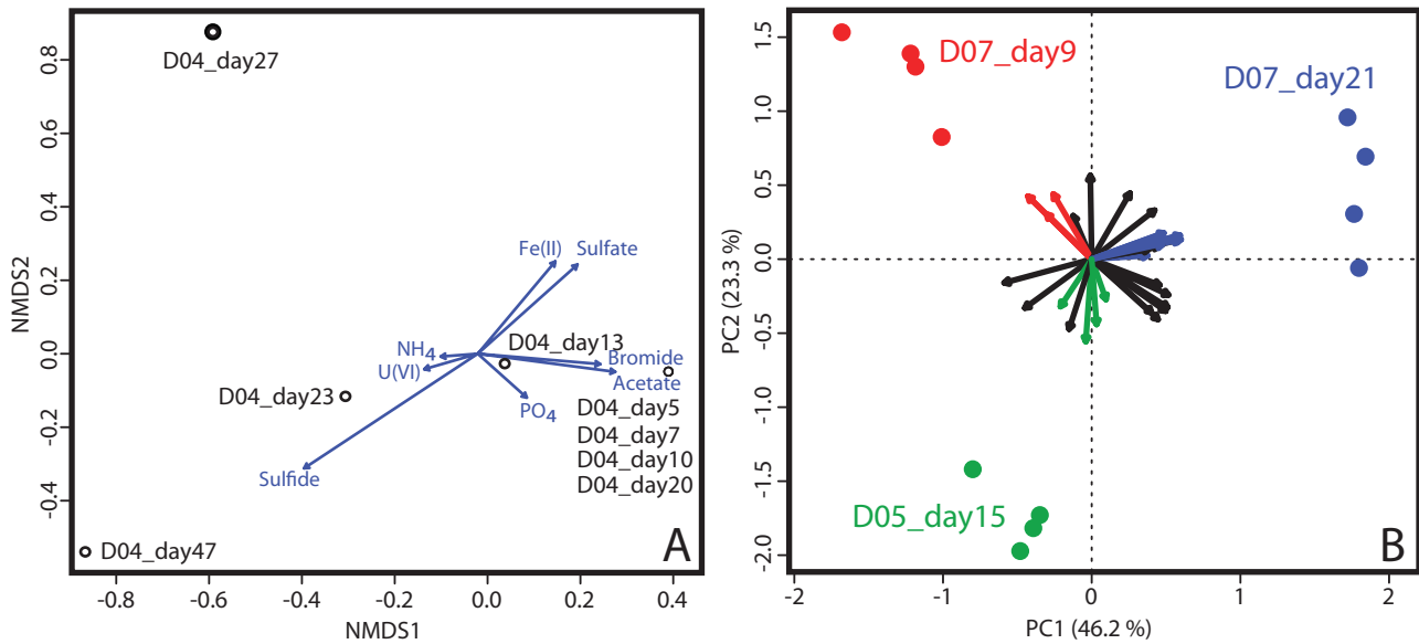
Fig. 4. A. Non-metric multidimensional scaling diagram showing clustering of 2008 samples using both conserved 'biomarker' and unique peptide abundances. Environmental vectors have been added illustrating the correlations between the clustering patterns of the biomass samples and geochemical gradients.
