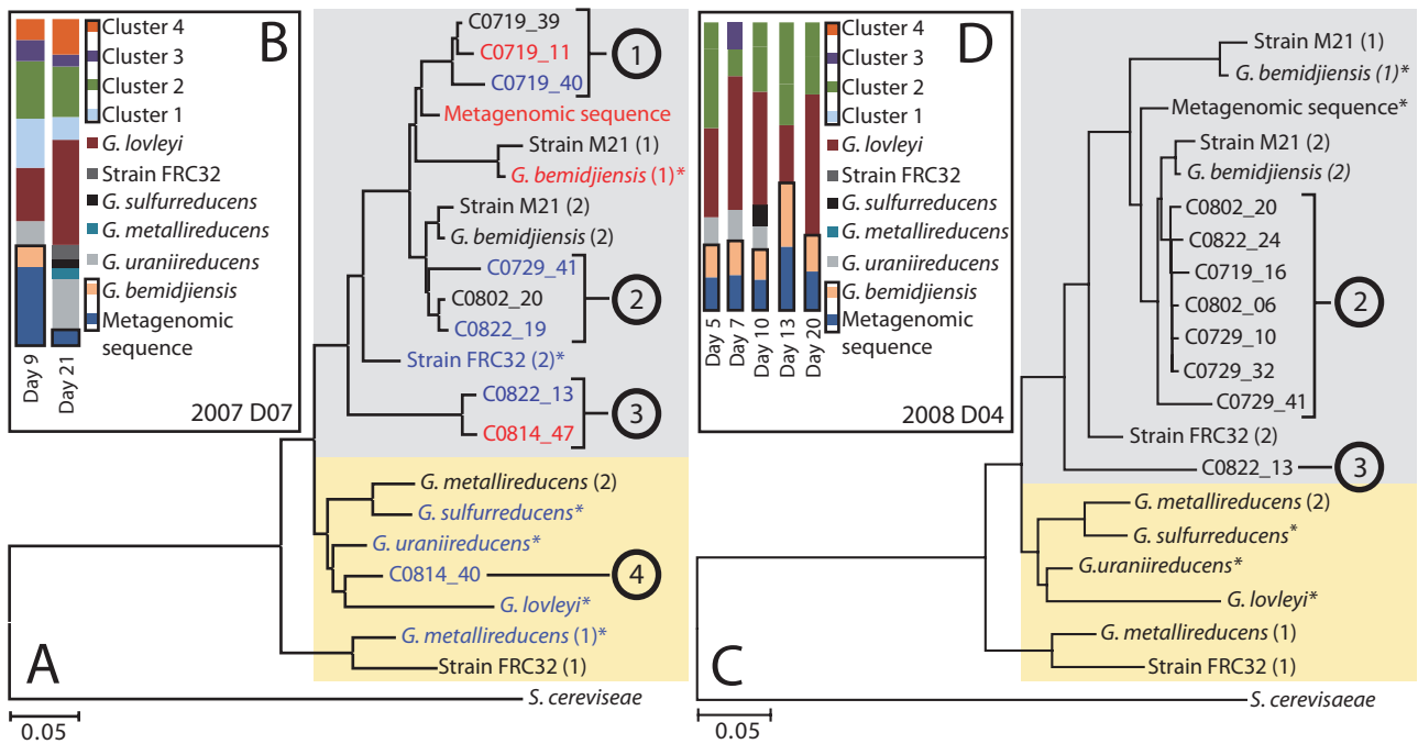
Fig. 5. A. A neighbour-joining tree constructed from aligned citrate synthase sequences for which unique peptides were detected in the 2007 data. Isolate sequences are included for reference. Peptides were detected for those isolate sequences marked by an asterisk '*'. Red and blue labels indicate sequences for which unique peptides were detected in only one of the samples (Red = D07_day9, Blue = D07_day21). Isolate CS identifications are as follows; G. bemidjiensis (1), gi145617433; G. bemidjiensis (2), gi145620657; Strain M21 (1), gm829064; Strain M21 (2), gm826531; Strain FRC32 (1), gi110599265; Strain FRC32 (2), gi110600278; G. lovleyi , gi118746732; G. sulfurreducens , gi39996208; G. uraniireducens , gi148263639; G. metallireducens (1), gi78222340; G. metallireducens (2), gi78223885. B. Peptide % abundances for all unique peptides matched against the citrate synthase database in samples D07_day9 and D07_day21 from the 2007 experiment. C. A neighbour-joining tree constructed from aligned citrate synthase sequences detected in the 2008 data. Isolate sequences are included for reference. Peptides were detected for those isolate sequences marked by an asterisk '*'. Geobacter CS identifications are as above. D. Peptide % abundances for all unique peptides matched against the citrate synthase database in samples D04_day5 through D04_day20 from the 2008 experiment. Saccharomyces cerevisiae was used as an out-group for the trees. The scale bar indicates the number of changes inferred as having occurred along each branch.
