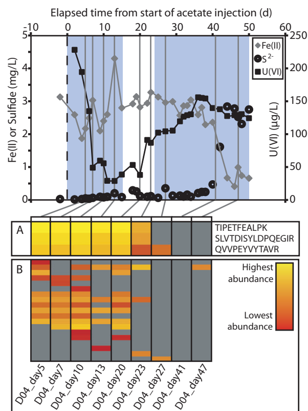
Fig. 3. Geochemical profiles for U(VI), Fe(II) and S^{2-} in well D04 during the 2008 biostimulation experiment. Heat-map abundances are shown for both the (A) conserved 'biomarker' peptides and (B) unique peptides matching CS proteins in all nine samples. Light blue zones show time periods of acetate injection. Uranium rebounds starts at -day 20.
