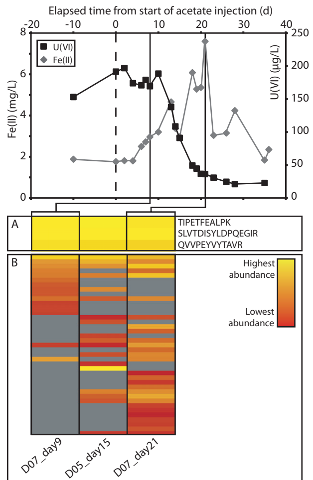
Fig. 2. Geochemical profiles for U(VI) and Fe(II) in well D07 during the 2007 biostimulation experiment. Heat-map abundances are shown for both the (A) conserved 'biomarker' peptides and (B) unique peptides matching CS proteins in all three samples.
