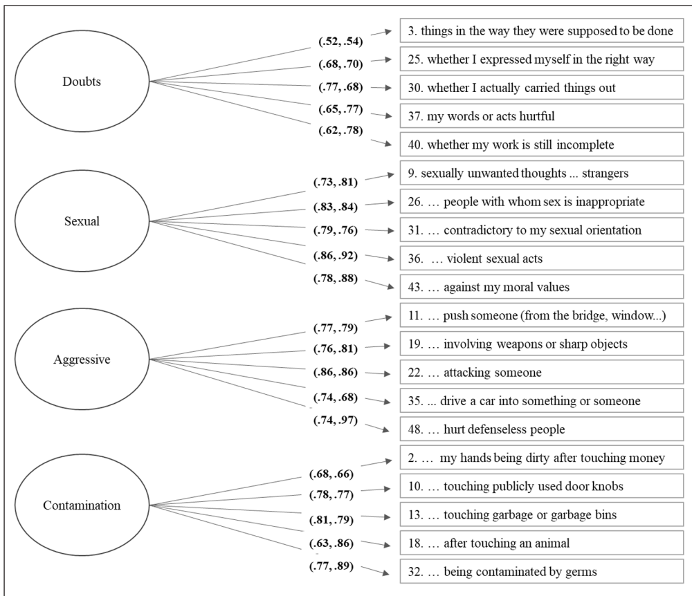
Figure 1: Standardized parameter estimates for Turkish and Belgian LOII-R factor model (Model3). Numbers in parentheses are Turkish followed by Belgian loading estimates; all parameter estimates are significant at p < .001 .
