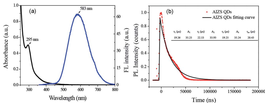
Fig. 1 (a) Absorption and photoluminescence spectra of AIZS QDs (concentration of 2 \times 10^{-4} mol \text{L}^{-1} ). The related absorption and fluorescence peak positions were 295 nm and 583 nm, respectively. (b) PL decay profile of AIZS QDs. \tau_1 , \tau_2 , and \tau_3 were 19.26, 22.53, and 19.25 \mu\text{s} , respectively. The average lifetime was 20.43 \mu\text{s} .
