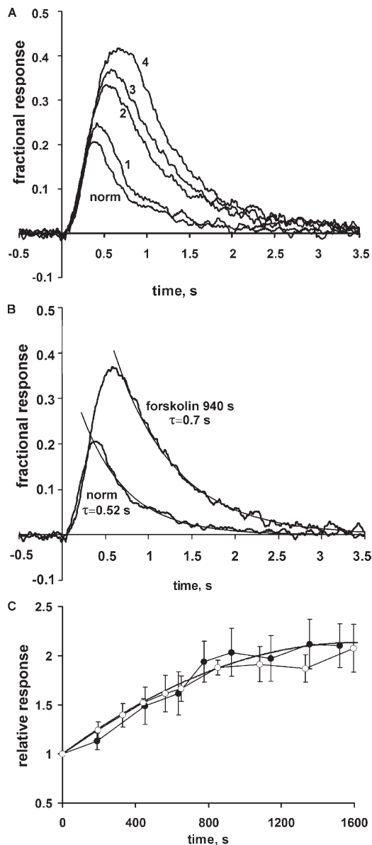
Figure 2. 2 \mu M forskolin increases photoreceptor sensitivity. (A) Responses at various time of incubation in forskolin-containing Ringer's solution. Response labeled "norm" was recorded in normal Ringer's solution just before the start of forskolin perfusion; 1–4 were recorded from the same cell after incubation with forskolin during 205, 610, 940, and 1,340 s, respectively. Flash intensity in all records was 0.82 \text{ photons} \cdot \mu\text{m}^{-2} per flash. Responses are normalized to corresponding dark current that was 19 pA in normal solution and 18 pA at the end of perfusion with forskolin. Each trace is the average of eight responses. (B) A single-exponential fit of the falling phase of two photoresponses recorded in normal solution and in the presence of forskolin after 940 s of incubation. Same cell as in A. (C) Changes of rods' sensitivity during incubation in forskolin-containing Ringer's solution, in configuration inner segment in (○) and outer segment in (●). The site of the forskolin application has no effect either on the time course or the magnitude of the response. The sensitivity is measured by photoresponses to a weak flash. All individual responses are normalized first to corresponding dark current, and second to corresponding response in normal Ringer's solution. Initial normalized response amplitudes were \approx 0.2 . The same flash
