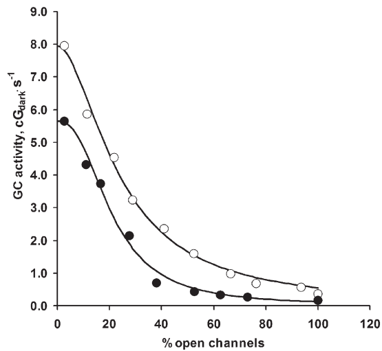
Figure 5. Forskolin modifies \text{Ca}^{2+} regulation of GC. GC activity in normal ( \circ ) and forskolin-containing ( \bullet ) solution versus fraction of open channels. Here, “100% open channels” refers to the situation in dark. The same cell as in Fig. 4 A. The lines are drawn using the Hill equation with K_{\text{cyc}} = 24\% and n = 1.8 in normal solution and K_{\text{cyc}} = 20.9\% and n = 2.5 in forskolin-containing solution.
