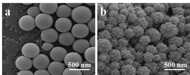
Fig. 8 SEM images of as-obtained particles (a) without MPS, (b) with MPS.
