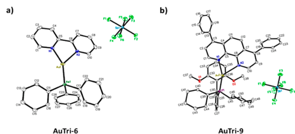
Figure 2. X-ray crystal structures: (a) structure of AuTri-6 and (b) structure of AuTri-9 . Outer-sphere solvent molecules are omitted for clarity. Thermal ellipsoids are shown at the 50% probability level.
