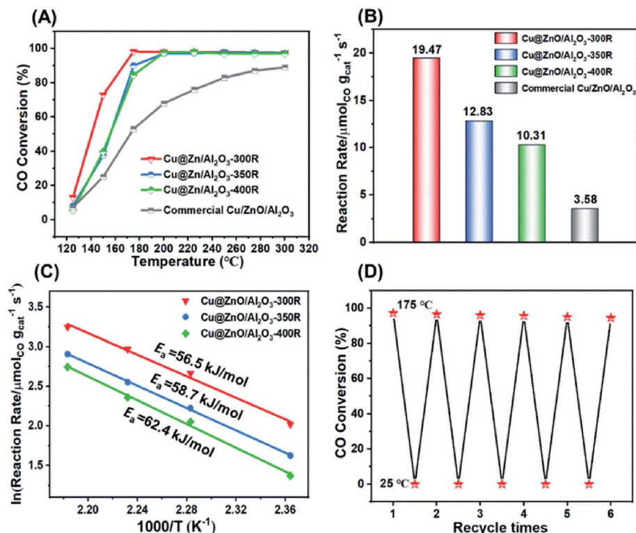
Fig. 2 (A) CO conversion as a function of reaction temperature over the Cu@ZnO/Al 2 O 3 catalysts as well as the commercial Cu/ZnO/Al 2 O 3 catalyst (WGS reaction conditions: 6% CO, 25% H 2 O, 69% Ar; WHSV: 15 700 mL g cat -1 h -1 ). (B) Reaction rates of the Cu@ZnO/Al 2 O 3 catalysts and the commercial Cu/ZnO/Al 2 O 3 catalyst at 175 °C. (C) Arrhenius plots of the WGS reaction over the three Cu@ZnO/Al 2 O 3 samples. (D) CO conversion vs. recycle times over the Cu@ZnO/Al 2 O 3 -300R catalyst (WGS reaction conditions: 6% CO, 25% H 2 O, 69% Ar; WHSV: 15 700 mL g cat -1 h -1 ).
