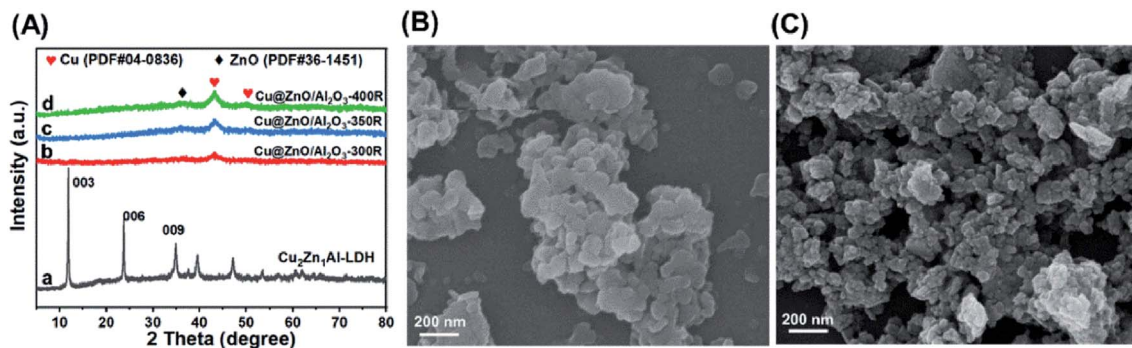
Fig. 1 XRD patterns of (a) \text{Cu}_2\text{ZnAl-LDH} precursor, (b) \text{Cu@ZnO/Al}_2\text{O}_3\text{-300R} , (c) \text{Cu@ZnO/Al}_2\text{O}_3\text{-350R} , and (d) \text{Cu@ZnO/Al}_2\text{O}_3\text{-400R} . (B) SEM image of \text{Cu}_2\text{ZnAl-LDH} precursor. (C) SEM image of reduced \text{Cu@ZnO/Al}_2\text{O}_3\text{-300R} .
