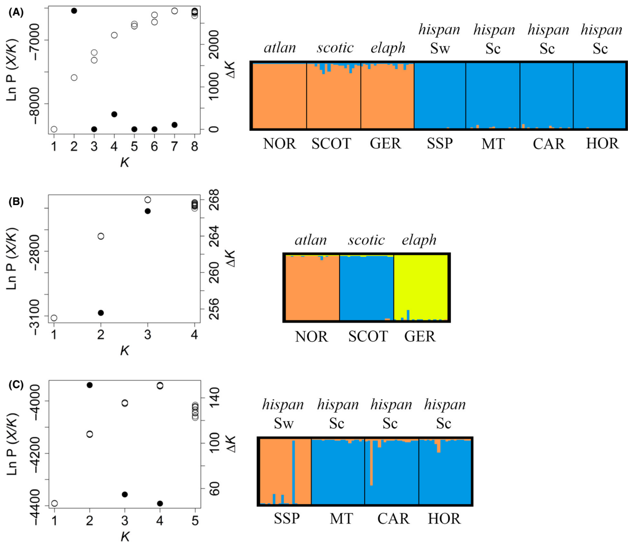
Figure 5. STRUCTURE software results. (A) All populations. Graph shows the log-likelihood values, \text{Ln Pr}(X/K) (white points) and Ad hoc statistic \Delta K (black points) showing the most probable number of genetic clusters ( K ). Membership coefficients of probability for each cluster are also showing. (B) Non-Spanish populations. (C) Spanish populations. NOR: Norway; SCOT: Scotland; GER: Germany; SSP: Sierra de San Pedro; MT: Montes de Toledo; CAR: Cardeña; HOR: Hornachuelos. Different subspecies are coded with the following notation: atlan : C. e. atlanticus ; scotic : C. e. scoticus ; elaph : C. e. elaphus ; hispan : C. e. hispanicus .
