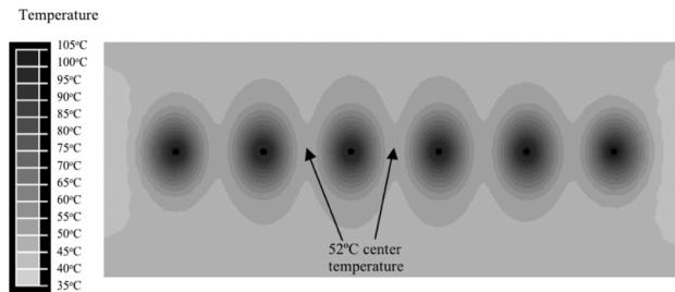
Fig. (6). Array of six needle electrodes at 1.5 cm distance, with voltage applied in monopolar mode (same voltage to all electrodes). Figure shows temperature contour at 3 min. Center temperature of 52 °C (arrow) due to reduced inter-electrode heating.
