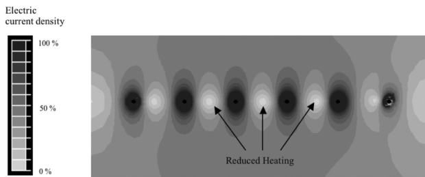
Fig. (7). Array of six needle electrodes at 1.5 cm distance, with voltage applied in monopolar mode (same voltage to all electrodes). Figure shows relative current density profile. Monopolar application results in reduced heating between electrodes (arrows) since electrodes are at same electrical potential.
