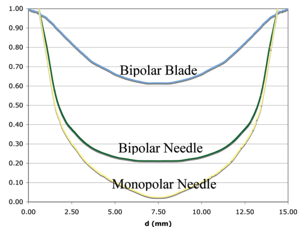
Fig. (10). Relative electric current density through center line between two electrodes (see Fig. 5) 15 mm apart. Blade electrodes with bipolar voltage application deposit power throughout the slice, while bipolar needle, and monopolar needle electrodes only produce heat close to the electrodes. Note that due to different electrode size, surfaces of needle electrodes are at x = 0.6 and 14.4 mm, and surfaces of blade electrodes are at x = 0.05 and 4.95 mm.
