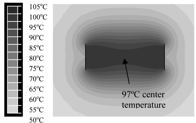
Fig. (9). Blade electrodes at 1.5 cm distance, with voltage applied in bipolar mode (between electrodes). Figure shows temperature contour at 3 min.
