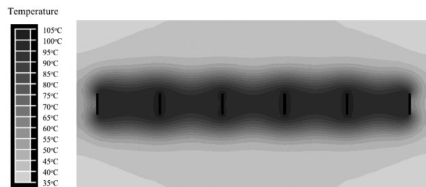
Fig. (11). Linear array of 6 blade electrodes at 1.5 cm distance. Voltage is rapidly switched between electrode pairs at 1 s intervals (see Fig. 4). Coagulation zone is ~1.5 cm wide after 3 min.
