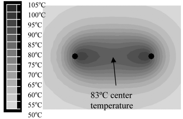
Fig. (8). Two needle electrodes at 1.5 cm distance, with voltage applied in bipolar mode (between electrodes). Figure shows temperature contour at 3 min.
