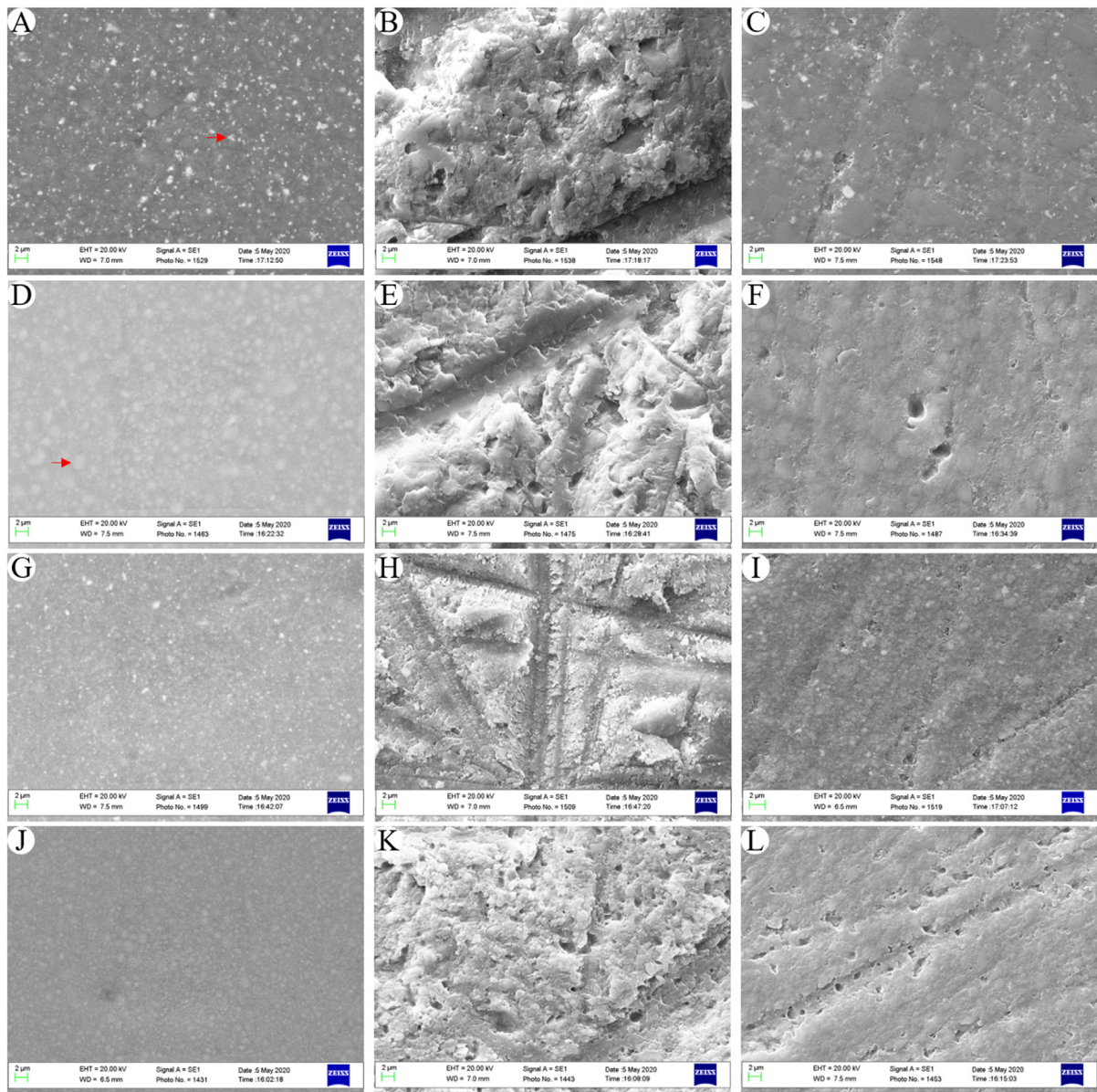
Figure 1 SEM images of all the groups. (A) HM-matrix strip group (red arrow indicates dispersed nanoparticles); (B) HM-sandpaper group; (C) HM-Sof-Lex group; (D) FT3-matrix strip group (red arrow indicates nanocluster); (E) FT3-sandpaper group; (F) FT3-Sof-Lex group; (G) TN-matrix strip group; (H) TN-sandpaper group; (I) TN-Sof-Lex group; (J) FT2-matrix strip group; (K) FT2-sandpaper group; (L) FT2-Sof-Lex group.
