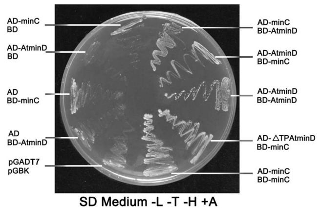
Figure 3 Interactions of EcMinC and AtMinD examined by yeast two hybrid analysis. Yeast cells grown without Leucine (L), Tryptophan (T) and Histidine (H), but with 3-AT. \Delta TP, deletion of the chloroplast transit peptide. SD, synthetic defined.
