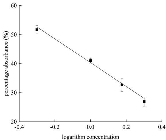
Fig. 1 Standard curve of AFB 1 .
