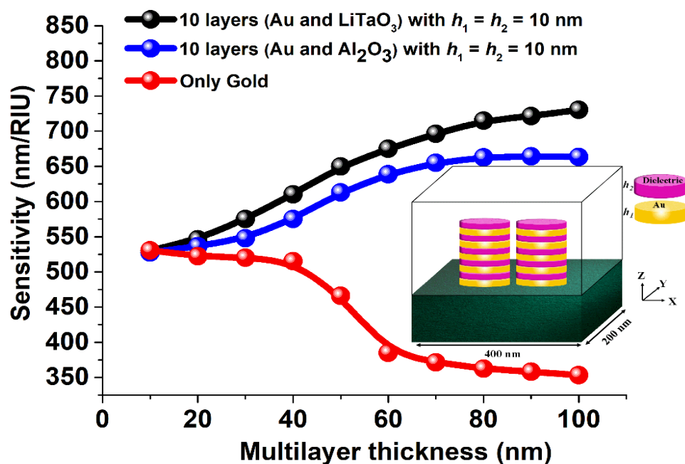
Figure 3. The sensitivity performance of a single metallic (Au) and \text{Al}_2\text{O}_3 and \text{LiTaO}_3 stacked antenna array when total height, h = 100 nm with or without stacking.
