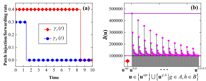
Figure 7. The experimental results in Example 2: (a) an optimal control, (b) a comparison between the optimal control and the set of static controls in terms of the energy efficiency.
