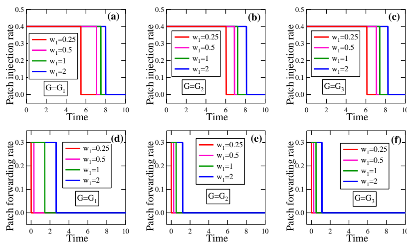
Figure 10. The experimental results in Experiment 1 about the effect of the loss coefficient on the optimal patching rate. (a) Patch injection rate, G = G_1 ; (b) Patch injection rate, G = G_2 ; (c) Patch injection rate, G = G_3 ; (d) Patch forwarding rate, G = G_1 ; (e) Patch forwarding rate, G = G_2 ; (f) Patch forwarding rate, G = G_3 .
