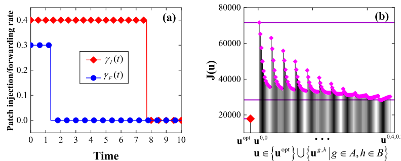
Figure 5. The experimental results in Example 1: (a) an optimal control, (b) a comparison between the optimal control and the set of static controls in terms of the energy efficiency.
