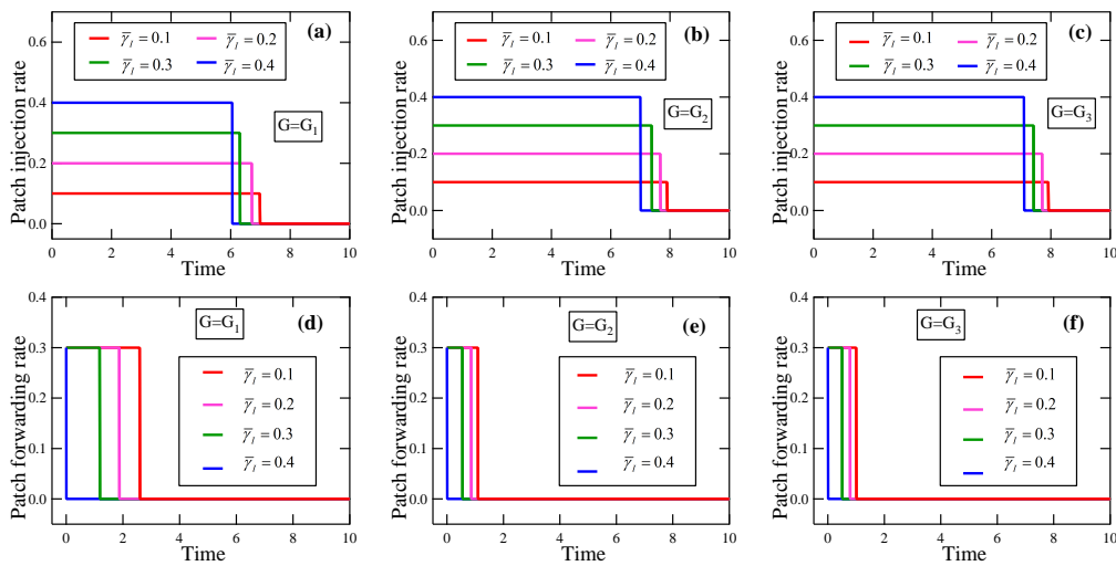
Figure 12. The experimental results in Experiment 2 about the effect of the maximum allowable patch injection rate on the optimal patching strategy. (a) Patch injection rate, G = G_1 ; (b) Patch injection rate, G = G_2 ; (c) Patch injection rate, G = G_3 ; (d) Patch forwarding rate, G = G_1 ; (e) Patch forwarding rate, G = G_2 ; (f) Patch forwarding rate, G = G_3 .
