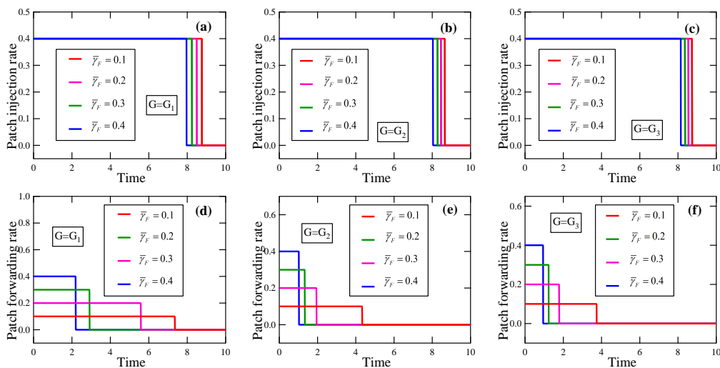
Figure 13. The experimental results in Experiment 2 about the effect of the maximum allowable patch forwarding rate on the optimal patching strategy. (a) Patch injection rate, G = G_1 ; (b) Patch injection rate, G = G_2 ; (c) Patch injection rate, G = G_3 ; (d) Patch forwarding rate, G = G_1 ; (e) Patch forwarding rate, G = G_2 ; (f) Patch forwarding rate, G = G_3 .
