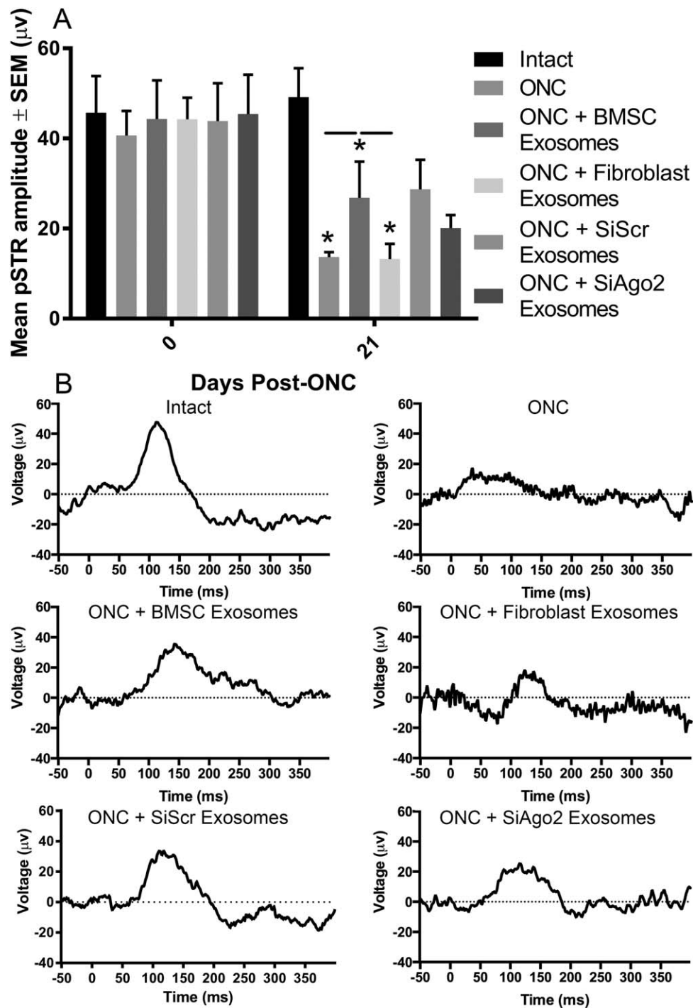
Figure 6. Figure 6: pSTR responses after ONC and exosome treatment. (A): Mean amplitude of pSTR from intact or ONC animals receiving intravitreal exosome treatments after receiving flash intensity of 1 \times 10^{-5} mcd/s. Black lines indicate significant difference between groups whereas asterisks indicate significant difference from the same group pre-ONC ( p < .05 ). (B): Representative traces of observable pSTR from groups 1-6. Abbreviations: ONC, optic nerve crush; pSTR, positive scotopic threshold response.
