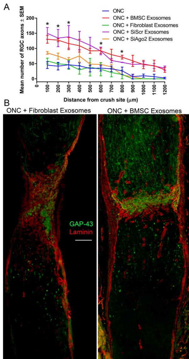
Figure 7. GAP-43 + RGC axon counts in the optic nerve after ONC. (A): Graph depicting the mean number of GAP-43 + RGC axons in the optic nerve at 100–1200 \mu\text{m} from the laminin + crush site. Asterisks indicate significant difference between ONC/ONC + fibroblast exosomes and ONC + BMSC exosomes/SiScr exosomes ( p < .05 ). (B): Representative images of optic nerves immunohistochemically stained for GAP-43 (green) and laminin (red) from groups 3 and 4 (scale bars: 100 \mu\text{m} ). Abbreviations: BMSC, bone marrow-derived mesenchymal stem cells; ONC, optic nerve crush; RGC, retinal ganglion cells.
