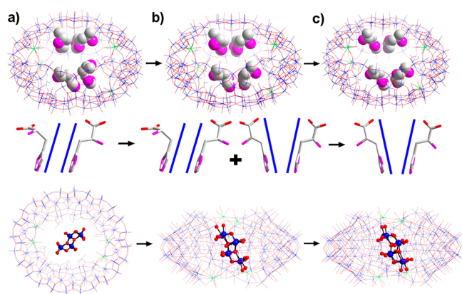
Figure 3. Evolution of \{\text{Mo}_{124}\text{Ce}_4\} as confined reaction vessel that is tuned by the arrangement of L-histidine. View of the parallel arrangement of L-histidine in \Lambda - 1a (a), parallel and V-shaped arrangement of L-histidine in 2a 1 (b), and V-shaped arrangement of L-histidine in 3a (c). Color code is the same as that in Figure 1.
