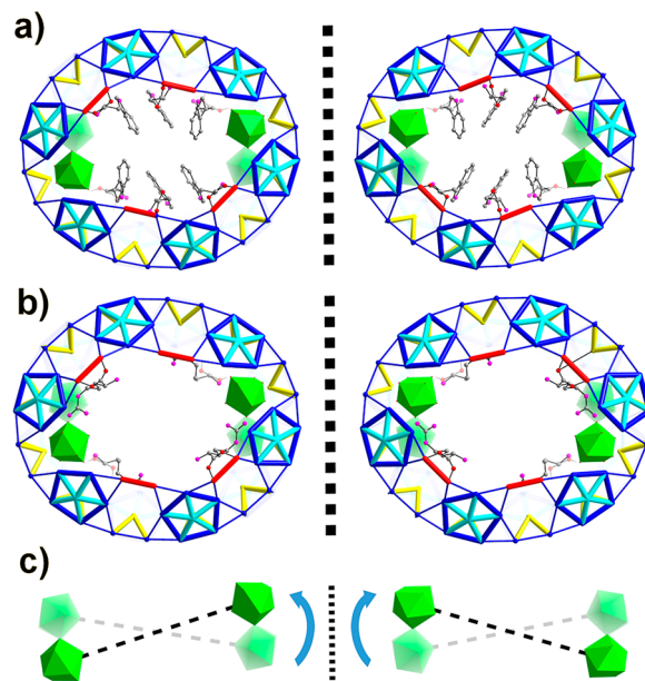
Figure 4. (a) View of the simplified framework of \Lambda - 4a (left) and \Delta - 4a (right) to highlight the basic \{\text{Mo}_8\} , \{\text{Mo}_2\} , and \{\text{Mo}_1\} building blocks. (b) View of the simplified framework of \Lambda - 5a (left) and \Delta - 5a (right). (c) Representation of the absolute configurations of \Lambda - 4a and \Lambda - 5a (left) and \Delta - 4a and \Delta - 5a (right) based on the helical arrangement of \text{Ce}^{3+} ions. The \text{Ce}^{3+} ions behind the plane is highlighted in transparency.
