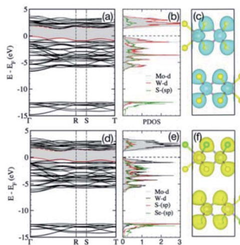
Fig. 5 Electronic band-structure, partial densities of states (states/eV-atom), and charge-density iso-surfaces (set to 0.08 \text{ eV \AA}^{-3} ) of (\text{Mo}_{0.5}\text{W}_{0.5})\text{S}_2 (a–c) and (\text{Mo}_{0.5}\text{W}_{0.5})\text{SSe}_2 (d, e), respectively. The indirect band gaps were calculated at 1.02 eV for (\text{Mo}_{0.5}\text{W}_{0.5})\text{S}_2 and 1.17 eV for (\text{Mo}_{0.5}\text{W}_{0.5})\text{SSe} . A 2 \times 2 \times 2 supercell was used to model W-disorder on Mo site with 24 atom cell (Mo = 4, W = 4, S = 16; and Mo = 4, W = 4, S = 8, Se = 8) atom per cell.
