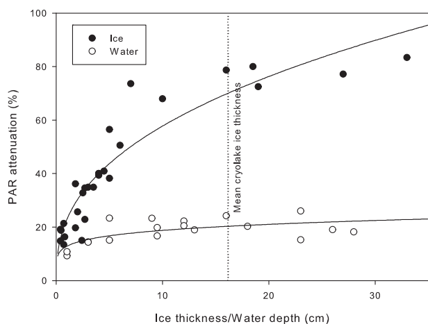
Figure 3. PAR attenuation (surface – subsurface) for ice lids of different thicknesses and with water depth on Joyce Glacier. Regression fit between ice thickness and PAR attenuation is \text{PAR} = 22.9 h_i^{0.40} , r^2 = 0.87 and water depth and PAR attenuation is \text{PAR} = 12.9 h_w^{0.14} , r^2 = 0.44 .
