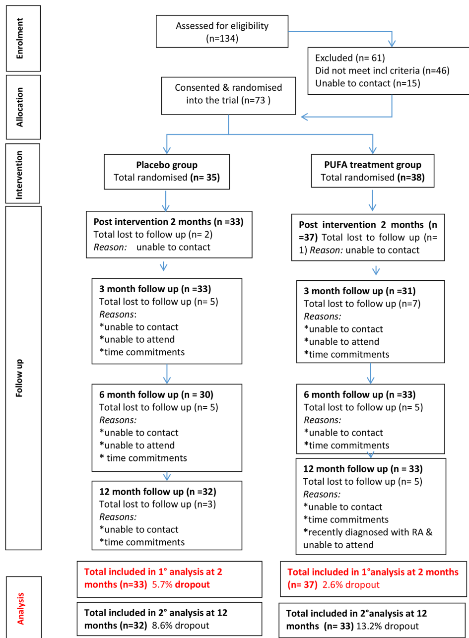
Figure 1 Consort diagram.
