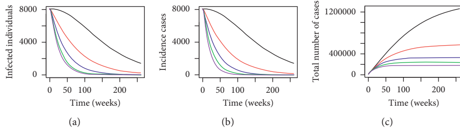
FIGURE 5: Numerical simulations for (a) infected individuals, (b) incidence cases (in weeks), and (c) total number of dengue cases in Malaysia where the black line: x = 0 , red line: x = 0.1 , blue line: x = 0.20 , green line: x = 0.30 , and purple line: x = 0.40 over a period of 5 years where P^* = 0.3450 .
