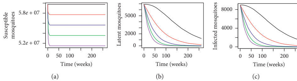
FIGURE 6: Dynamical behaviour for Aedes mosquitoes in Malaysia where the black line: x = 0 , red line: x = 0.1 , blue line: x = 0.20 , green line: x = 0.30 , and purple line: x = 0.40 over a period of 5 years where P^* = 0.3450 .
