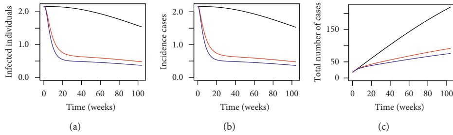
FIGURE 1: Numerical simulations for (a) infected individuals, (b) incidence cases (in weeks), and (c) cumulative total number of dengue cases within the trial site in Section 15 of Shah Alam, Selangor, Malaysia, for P = 0.1280 where the black line, red line, and blue line represent P^* = 0 , P^* = 0.3450 , and P^* = 0.4897 , respectively, over a period of 2 years.
