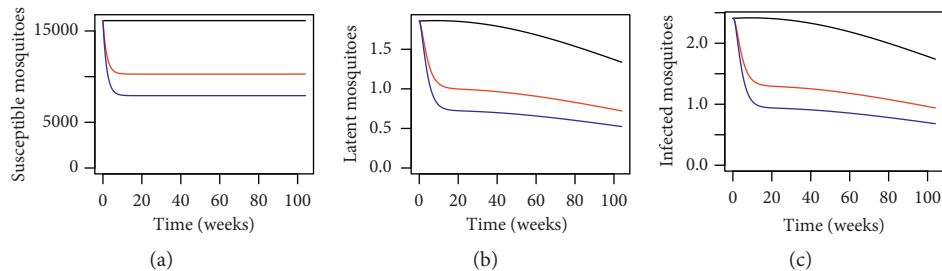
FIGURE 4: Dynamical behaviour for Aedes mosquitoes within the trial site in Section 15 of Shah Alam, Selangor, Malaysia, for P = 0.6610 where the black line, red line, and blue line represent P^* = 0 , P^* = 0.3450 , and P^* = 0.4897 , respectively, over a period of 2 years.
