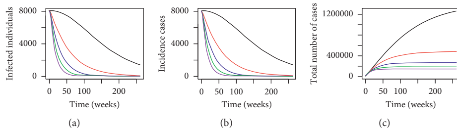
FIGURE 7: Numerical simulations for (a) infected individuals, (b) incidence cases (in weeks), and (c) total number of dengue cases in Malaysia where the black line: x = 0 , red line: x = 0.1 , blue line: x = 0.20 , green line: x = 0.30 , and purple line: x = 0.40 over a period of 5 years where P^* = 0.4897 .
