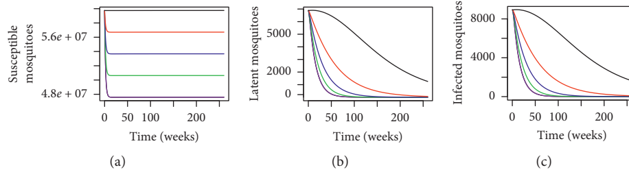
FIGURE 8: Dynamical behaviour for Aedes mosquitoes in Malaysia where the black line: x = 0 , red line: x = 0.1 , blue line: x = 0.20 , green line: x = 0.30 , and purple line: x = 0.40 over a period of 5 years where P^* = 0.4897 .
