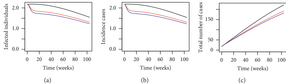
FIGURE 3: Numerical simulations for (a) infected individuals, (b) incidence cases (in weeks), and (c) cumulative total number of dengue cases within the trial site in Section 15 of Shah Alam, Selangor, Malaysia, for P = 0.6610 where the black line, red line, and blue line represent P^* = 0 , P^* = 0.3450 , and P^* = 0.4897 , respectively, over a period of 2 years.
