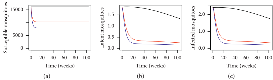
FIGURE 2: Dynamical behaviour for Aedes mosquitoes within the trial site in Section 15 of Shah Alam, Selangor, Malaysia, for P = 0.1280 where the black line, red line, and blue line represent P^* = 0 , P^* = 0.3450 , and P^* = 0.4897 , respectively, over a period of 2 years.
