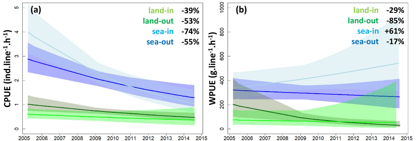
Fig 3. Trends in catch per unit effort (CPUE, a) and weight per unit effort (WPUE, b) of recreational fishermen fishing from land along the coastline (land) vs at sea from boats (sea), and inside (in) vs outside (out) the Cerbère-Banyuls marine reserve. Curves represent mean trajectories estimated by generalized linear models and shadings indicate 95% confidence intervals. The percent changes in mean CPUE and WPUE between the beginning and the end of the study period are provided as text on the plots. See S4 Table for mean and confidence interval values. Refer to S5 Table for parameter estimates.
