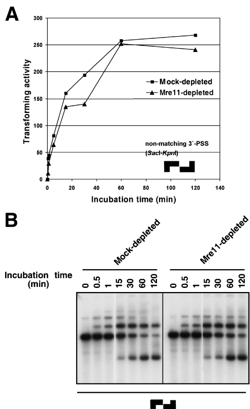
Figure 4. NHEJ kinetics is not affected by Mre11 depletion. Nonmatching 3'-PSS substrate SacI - KpnI was incubated in mock- and Mre11-depleted membrane-free cytosol, and samples were taken at the indicated time points. DNA was recovered and analyzed by (A) colony formation assay and (B) Southern blot hybridization (grouping of different segments of the same gel is indicated by dividing lines).
