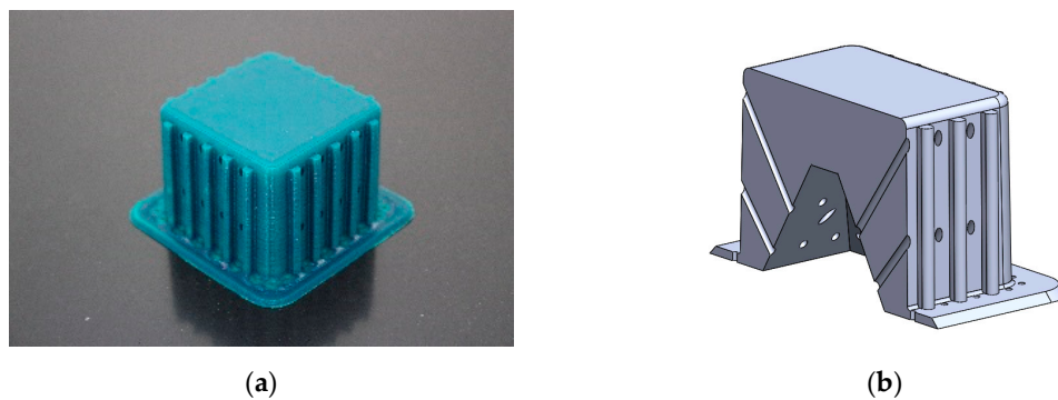
Figure 4. Example images of the mould used for thermoforming compression specimens: (a) image of the mould, (b) vacuum channels included inside the mould.
